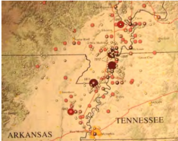
Map of New Madrid Fault Showing Years of Activity
